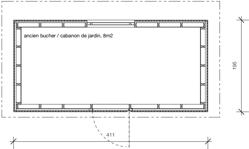
Plan 1 :50
